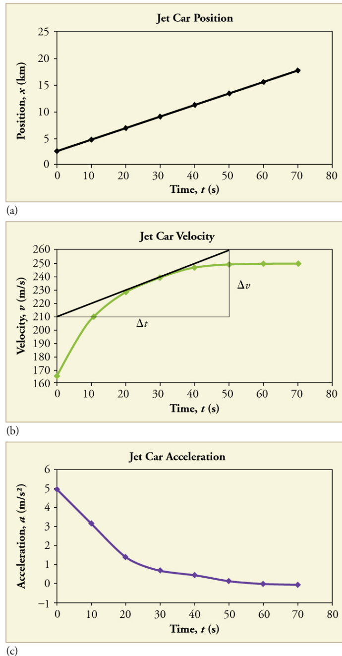
Figure 2.51 Graphs of motion of a jet-powered car as it reaches its top velocity. This motion begins where the motion in Figure 2.48 ends.
