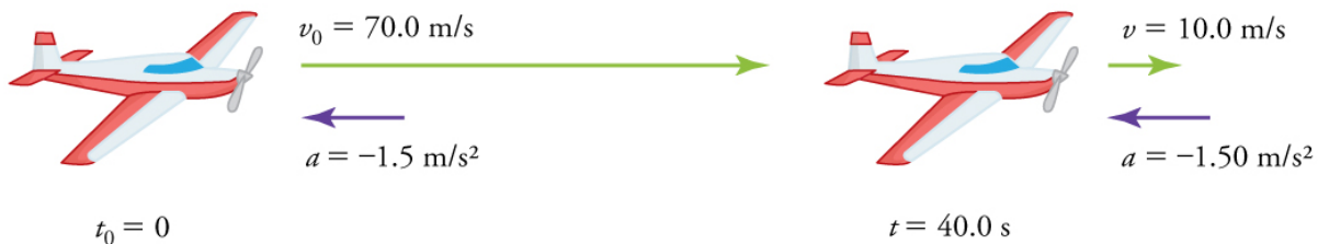
Figure 2.29 The airplane lands with an initial velocity of 70.0 \text{ m/s} and slows to a final velocity of 10.0 \text{ m/s} before heading for the terminal. Note that the acceleration is negative because its direction is opposite to its velocity, which is positive.
